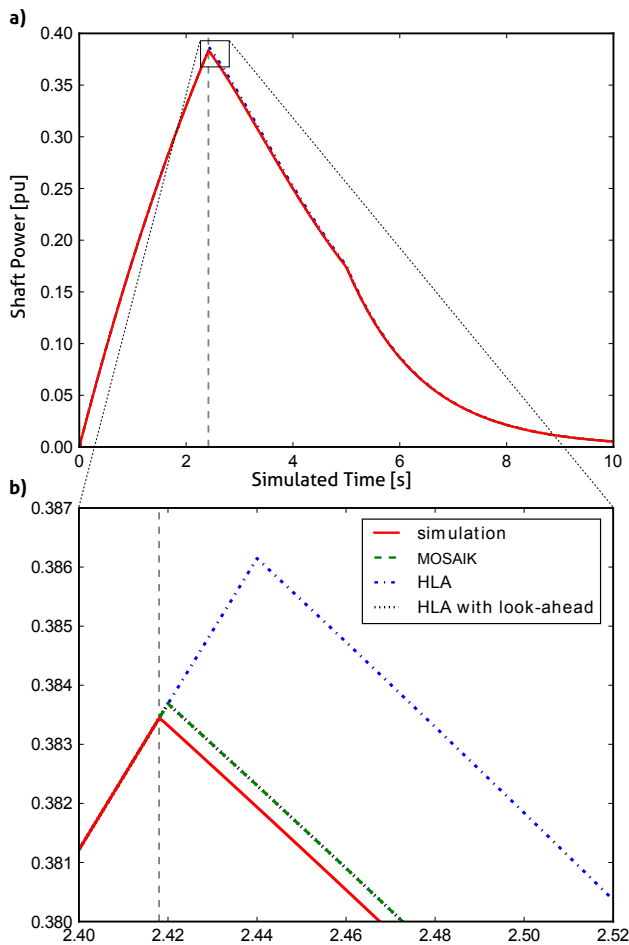
Fig. 3 Calculated wind power input to the turbine for different (co-)simulation setups. Full plot (a) and zoomed-in around the time of the event (b).
